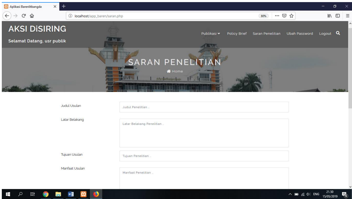
Gambar 5. Saran Penelitian
